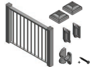
KNOCKDOWN GATE KIT (3-1/2" Posts - Maximum opening size 54")
